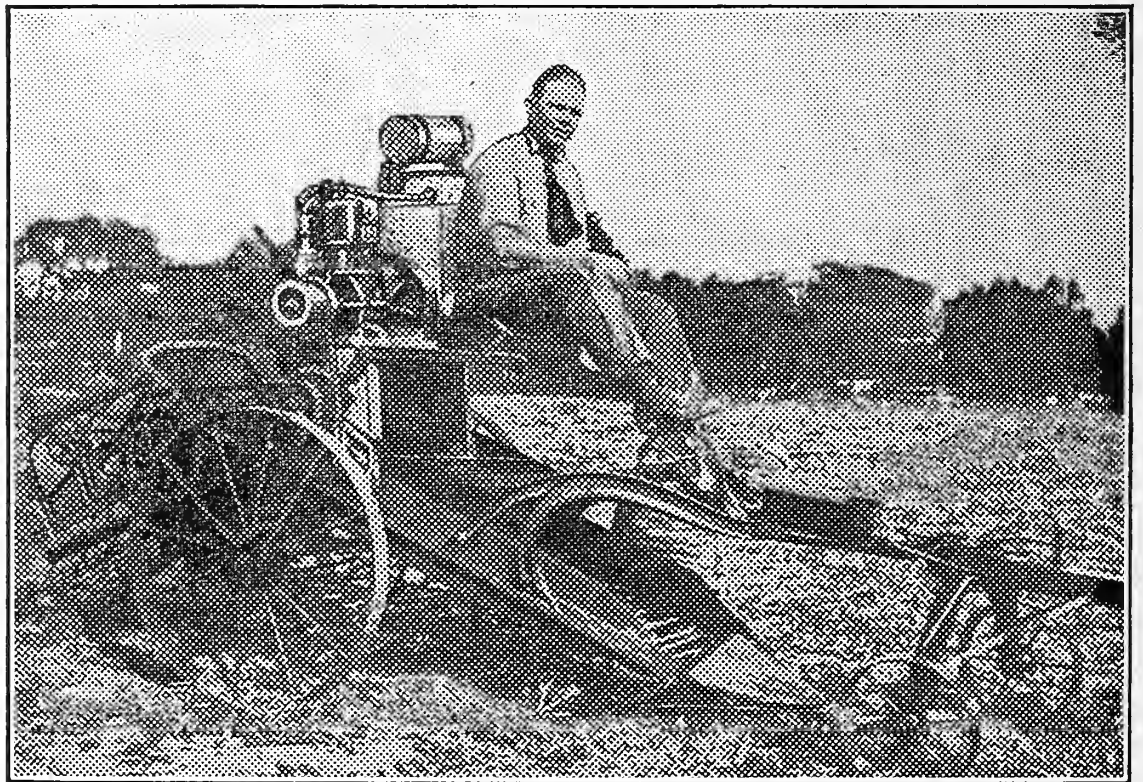
Four-Horsepower Cushman Engine on a Hoover Digger
